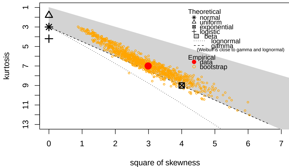
Figure 1: Skewness-kurtosis plot of nest distances from the shore in km.
