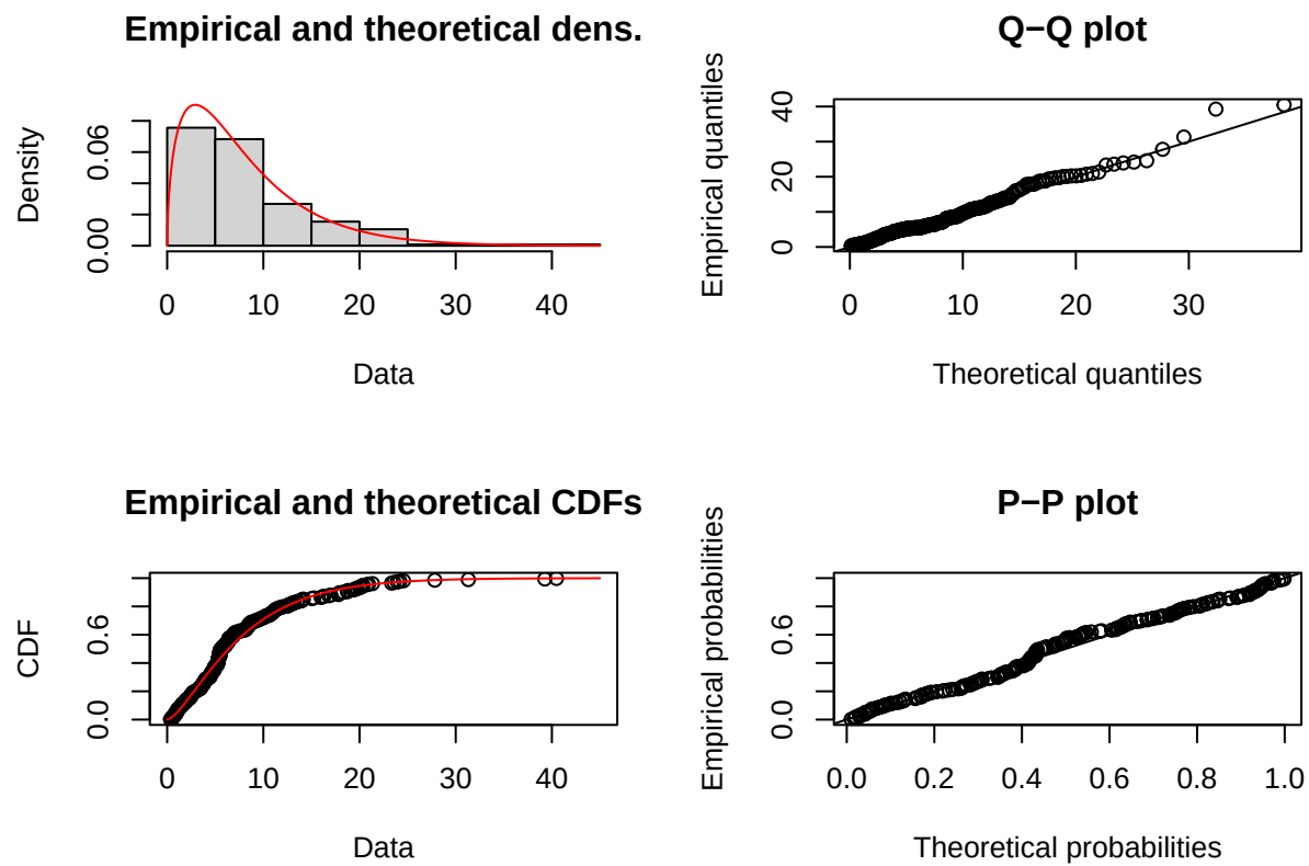
Figure 2: Nest gamma distribution fit diagnostics. The top-left plot shows the empirical distribution of nest data (grey bars) overlaid with the fitted density curve (red line). The x-axis is distance from the coast in km. The remaining plots show model fit diagnostics.
